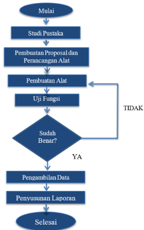
Gambar 4 Flowchart penelitian
