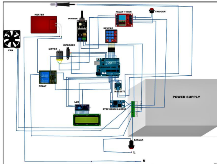
Figure 4. wiring diagram
