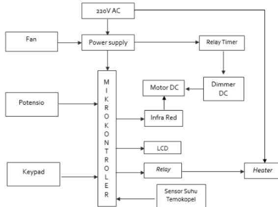
Figure 3. Block Diagram
